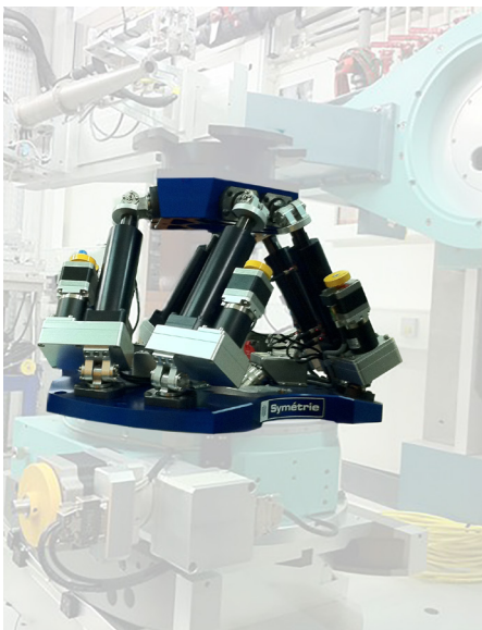
This hexapod positions a vacuum chamber containing a gas sample and offers a \pm 20^\circ angular range.
