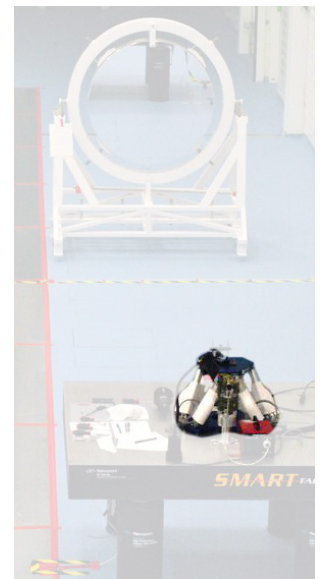
The BREVA hexapod is part of the ESA Star Tiger-2 test set-up to simulate a way to eclipse the Sun in space with two satellites flying in tight formation.
