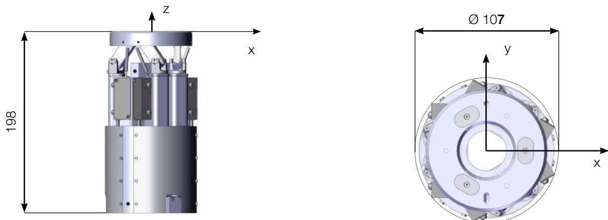
Hexapod in middle position
