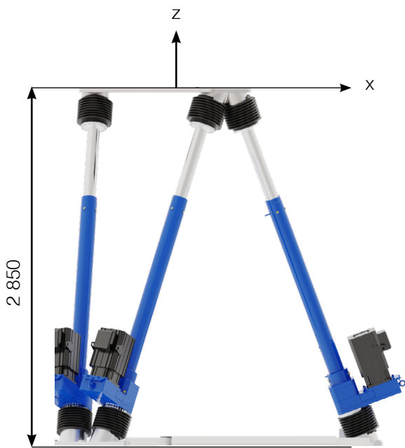
Hexapod in middle position
