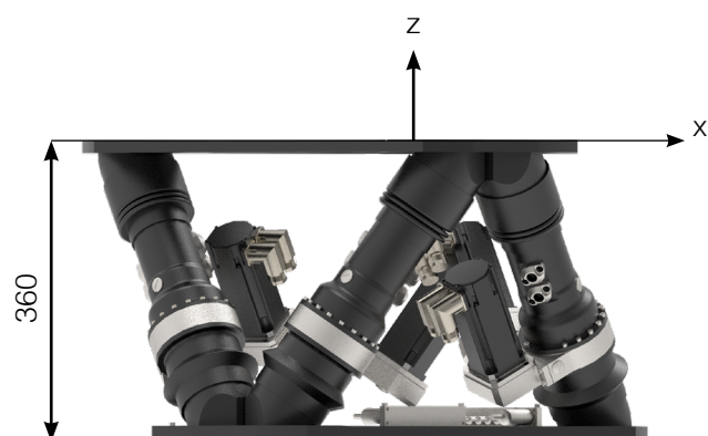
Hexapod in middle position
